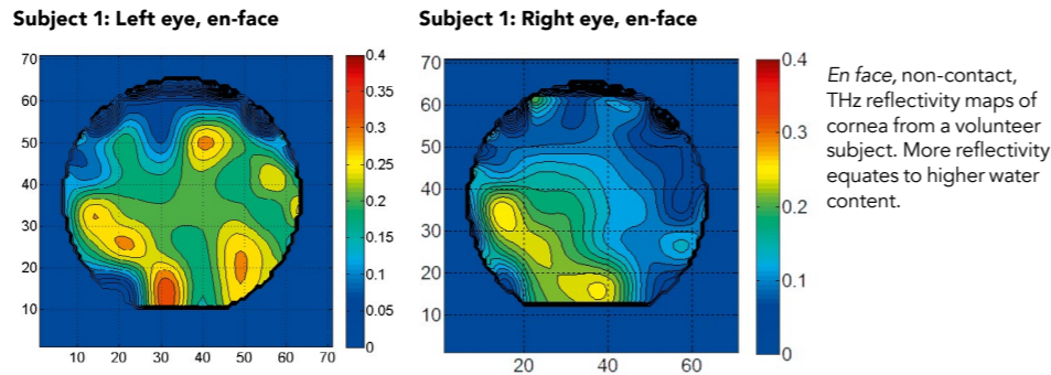
Reflectivity at 650GHz • Image acquisition time: ~20 seconds • Imaging subject stays completely stationary • Optics modification was crucial to imaging feasibility success
